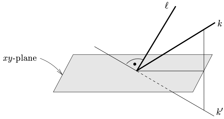
Figure 7: l is Minkowski-orthogonal to k .
