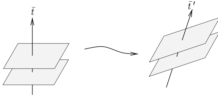
Figure 19: World-view transformation in three space-time dimensions, cf. Figures 15 and 16.
