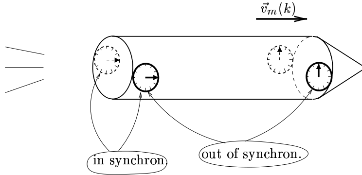
Figure 36: Clocks do not get out of synchronism orthogonal to movement. Imagine the little clocks glued to the hull of the spaceship.
