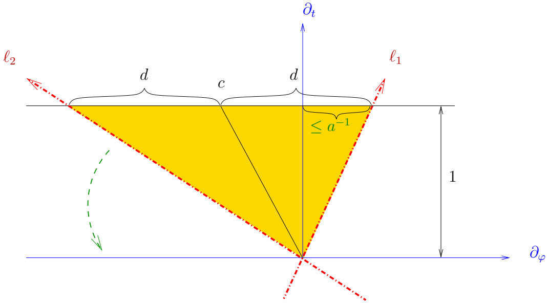
Figure 5: The light cone in the t\varphi -plane, between r_0 and r_1 . We draw the light cones with respect to the Killing vector fields \partial_t, \partial_\varphi . As we move towards the time machine region, i.e. towards r_1 , \ell_2 lowers to horizontal while \ell_1 is less than or equal a^{-1} .
