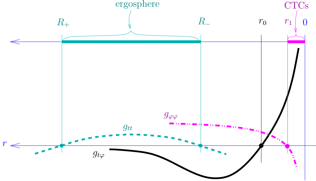
Figure 4: Illustration for the Kerr-Newman metric. The picture faithfully represents the order of the roots (i.e. zeros) of g_{t\varphi} , g_{tt} and g_{\varphi\varphi} and where these three functions are negative or positive; the picture does not faithfully represent the proportions of the distances and their magnitudes. The ergosphere and the “Time Machine” (where the CTCs are) are disjoint, and the light cone is erect between them at r_0 . In some sense, g_{t\varphi} represents the tilting of the light cones. See also Figure 3.
