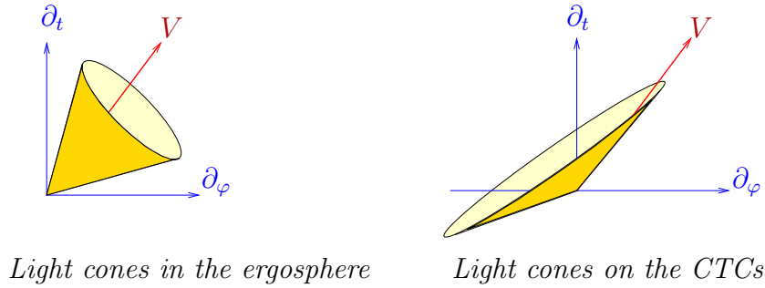
Figure 2: Light cones in the ergosphere and light cones on the CTCs look different.
