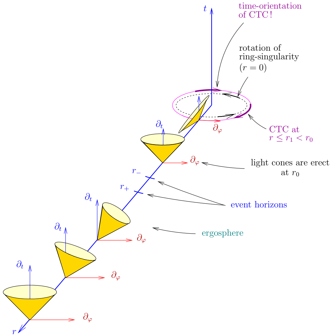
Figure 3: This is how light cones behave in Kerr-Newman spacetimes. For r_0, r_1 and computations see section 5, especially Figure 4.
